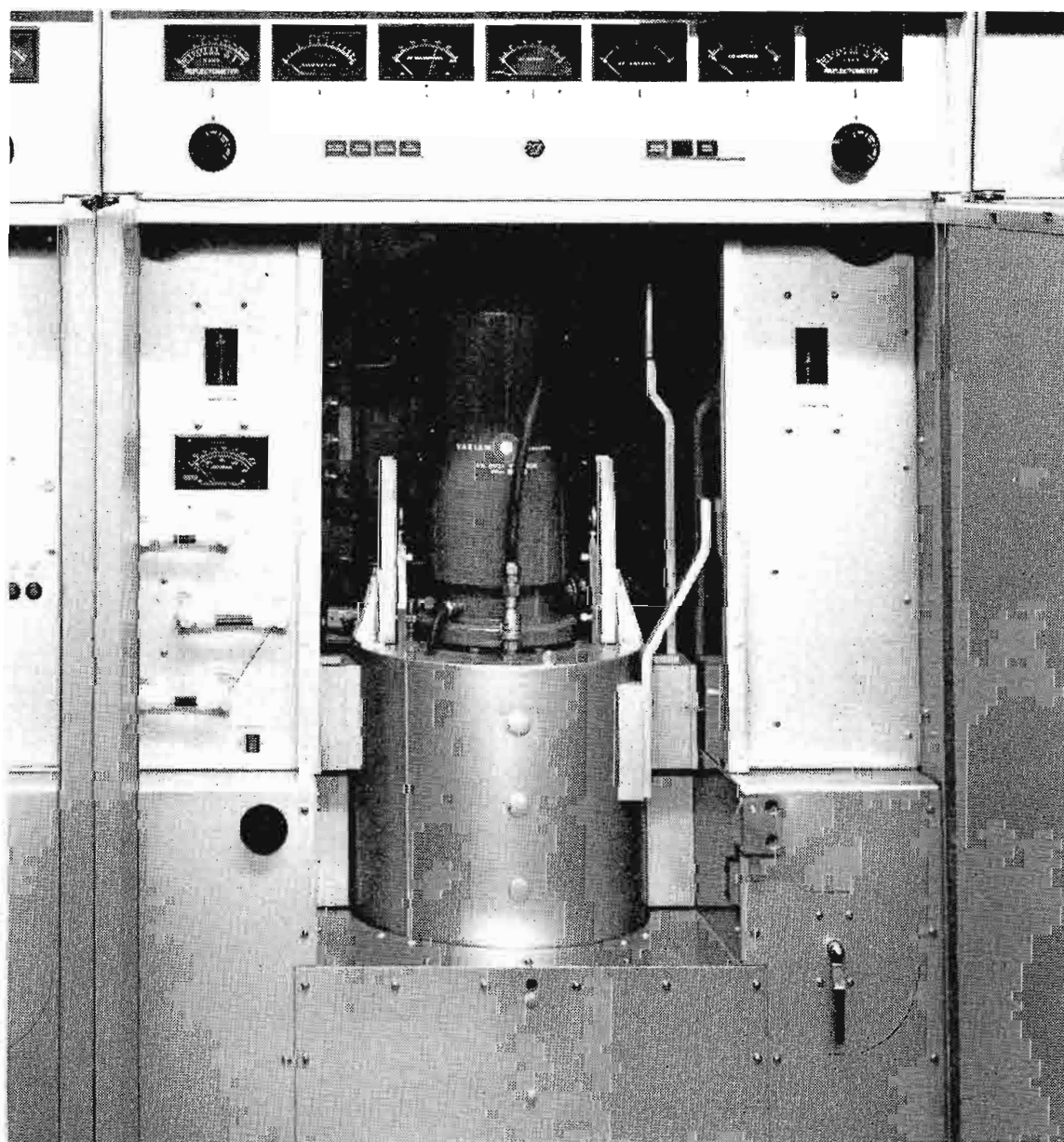
FIG. 3. View of one of diplexed visual cubicles. Coaxial patch panel shown at left permits instant use of a visual PA for the aural PA.
