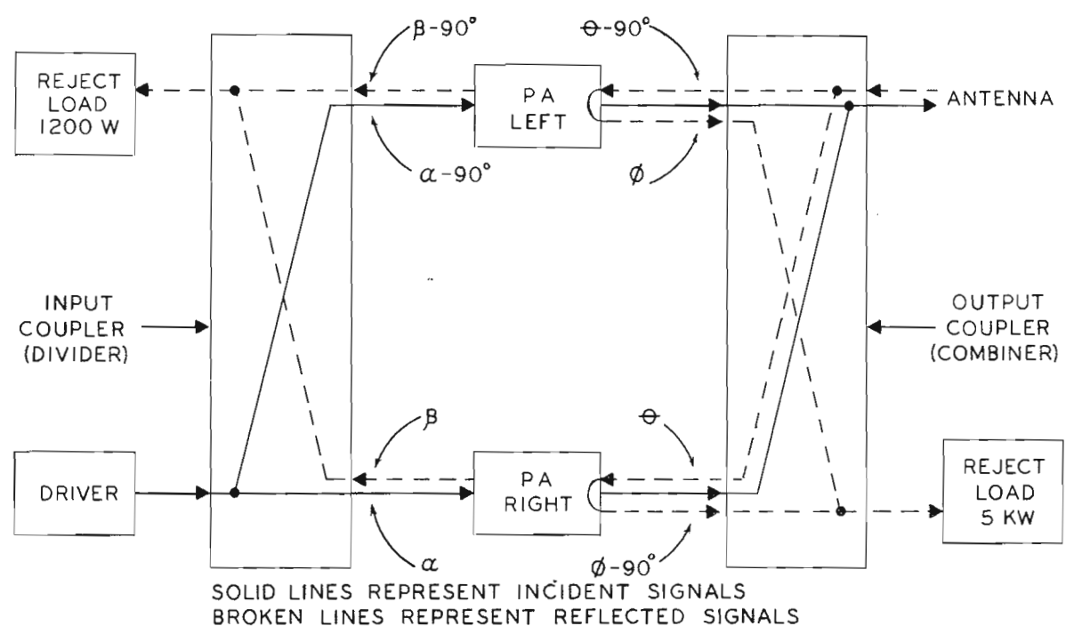
FIG. 2. The coaxial coupler used with the TT-25EL to combine the outputs of the diplexed power amplifiers.
