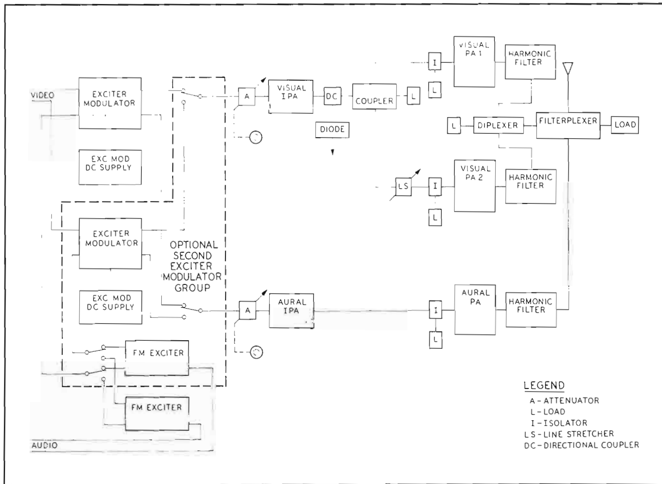
FIG. 2. TTU-110A block diagram. The optional spare exciter and modulator group is indicated by dashed lines. A spare IPA group is also available as an option if desired.
