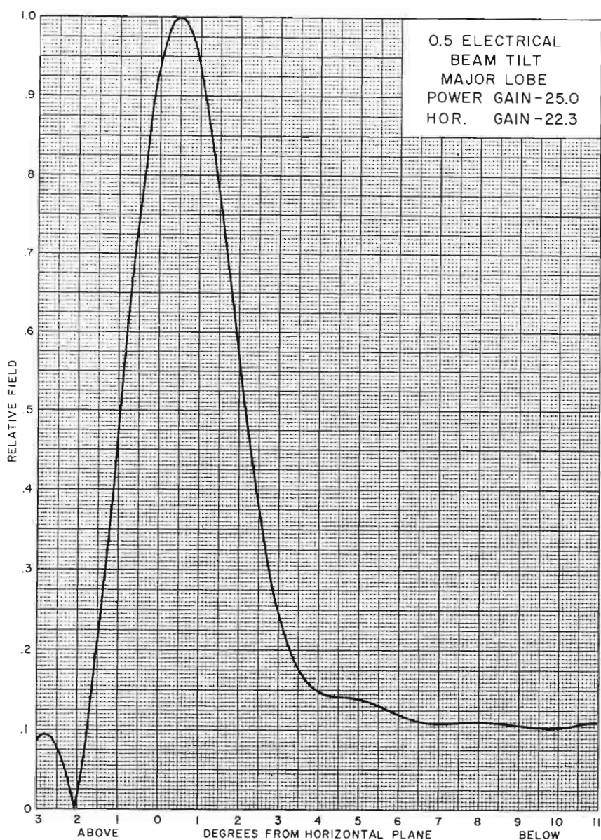
FIG. 9. Shaped vertical radiation pattern of TFU-25GA Pylon.
