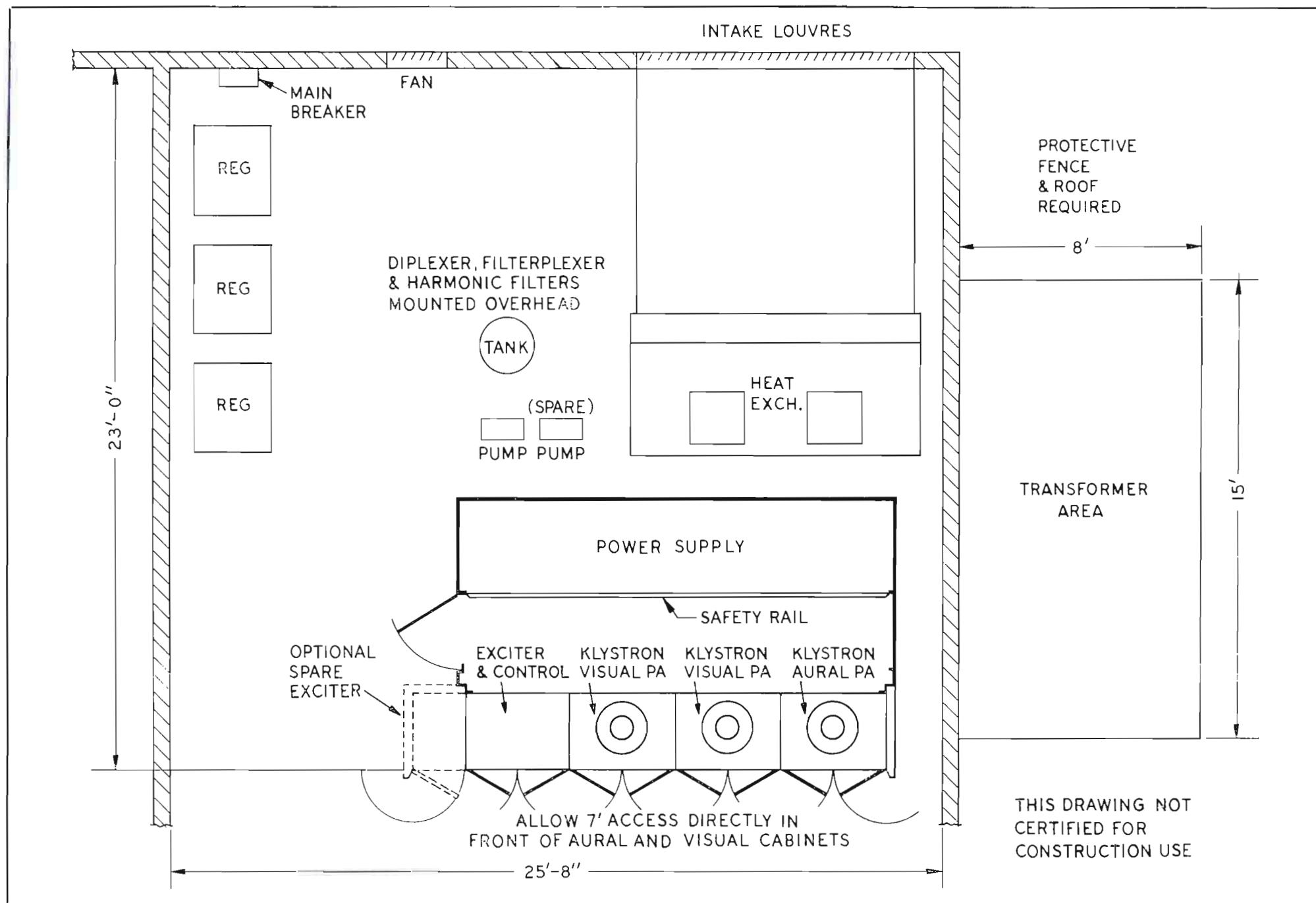
FIG. 7. Floor plan layout of TTU-110A transmitter offers considerable flexibility. Power supply may be located remotely, if desired.
