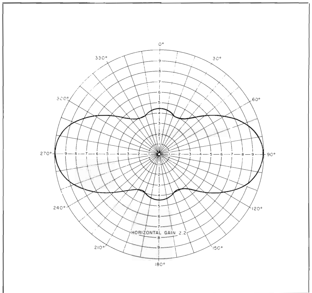
FIG. 10. Typical horizontal "peanut" pattern of UHF-TV Pylon.
