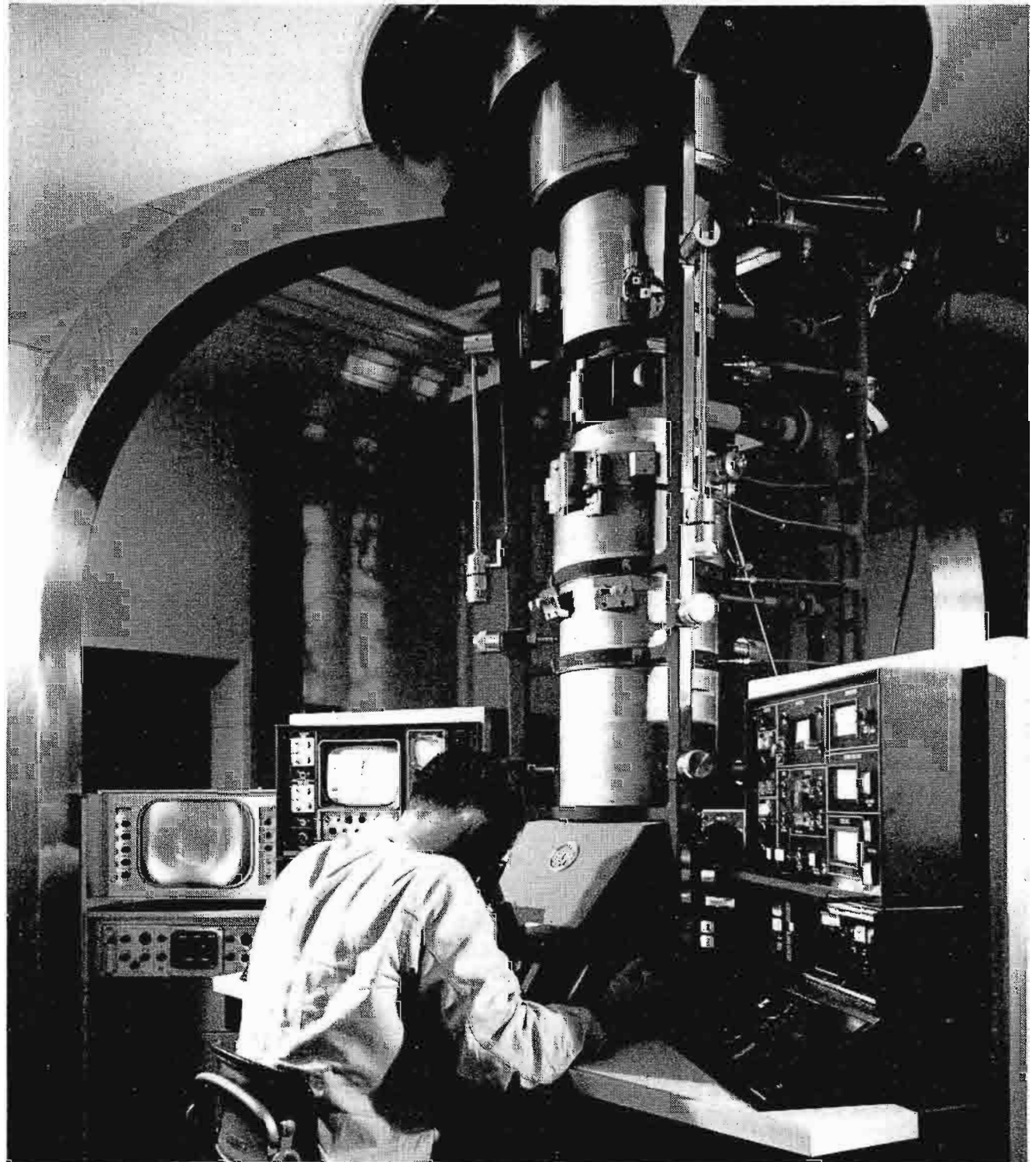
Million-volt instrument set to unlock metallurgical secrets for U.S. Steel researchers.
