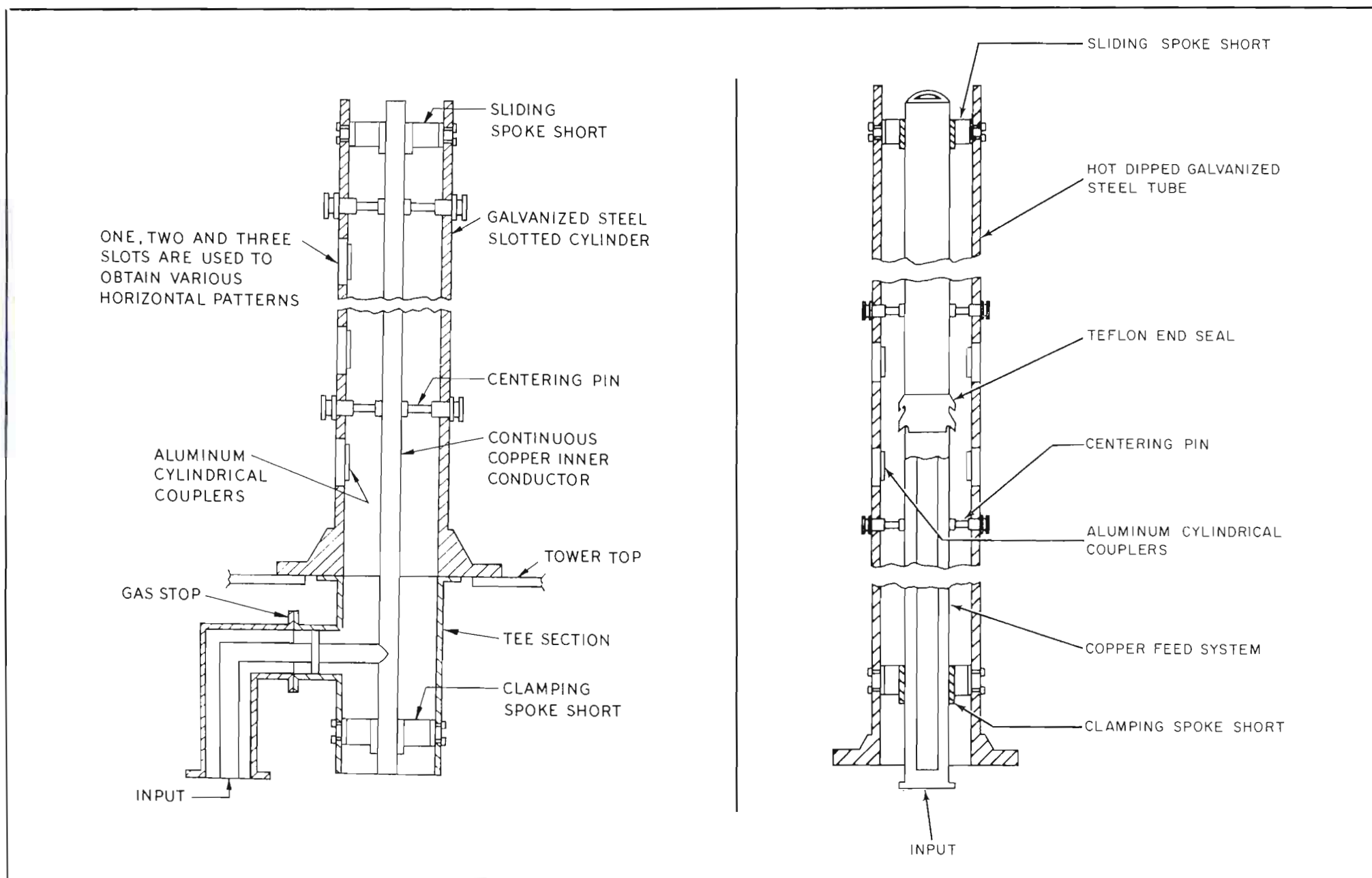
FIG. 13. Schematic diagrams showing end-fed Pylon, left, and center-fed Pylon, right. End-feed or "T-feed" is used to achieve high input power capabilities for directional antennas.
