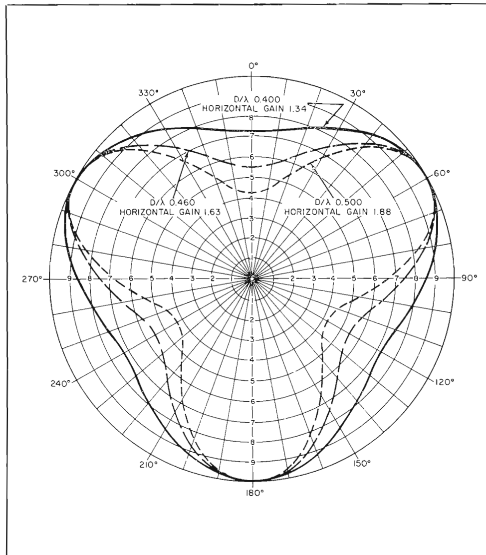
FIG. 12. Typical horizontal "tri-lobe" pattern of UHF-TV Pylon.
