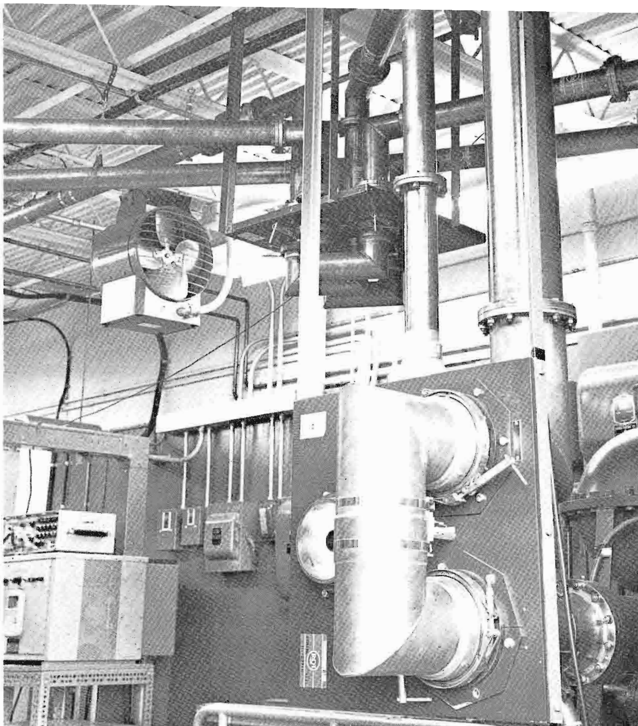
FIG. 12. Coaxial patch system at transmitter location. The 3½-inch patch at top center of photo is used to bypass the filterplexer. The 6½-inch patch in foreground is for connection of dummy load.
