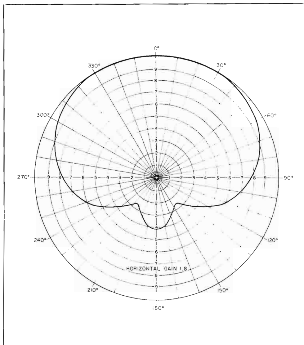
FIG. 11. Typical horizontal "skull" pattern of UHF-TV Pylon.
