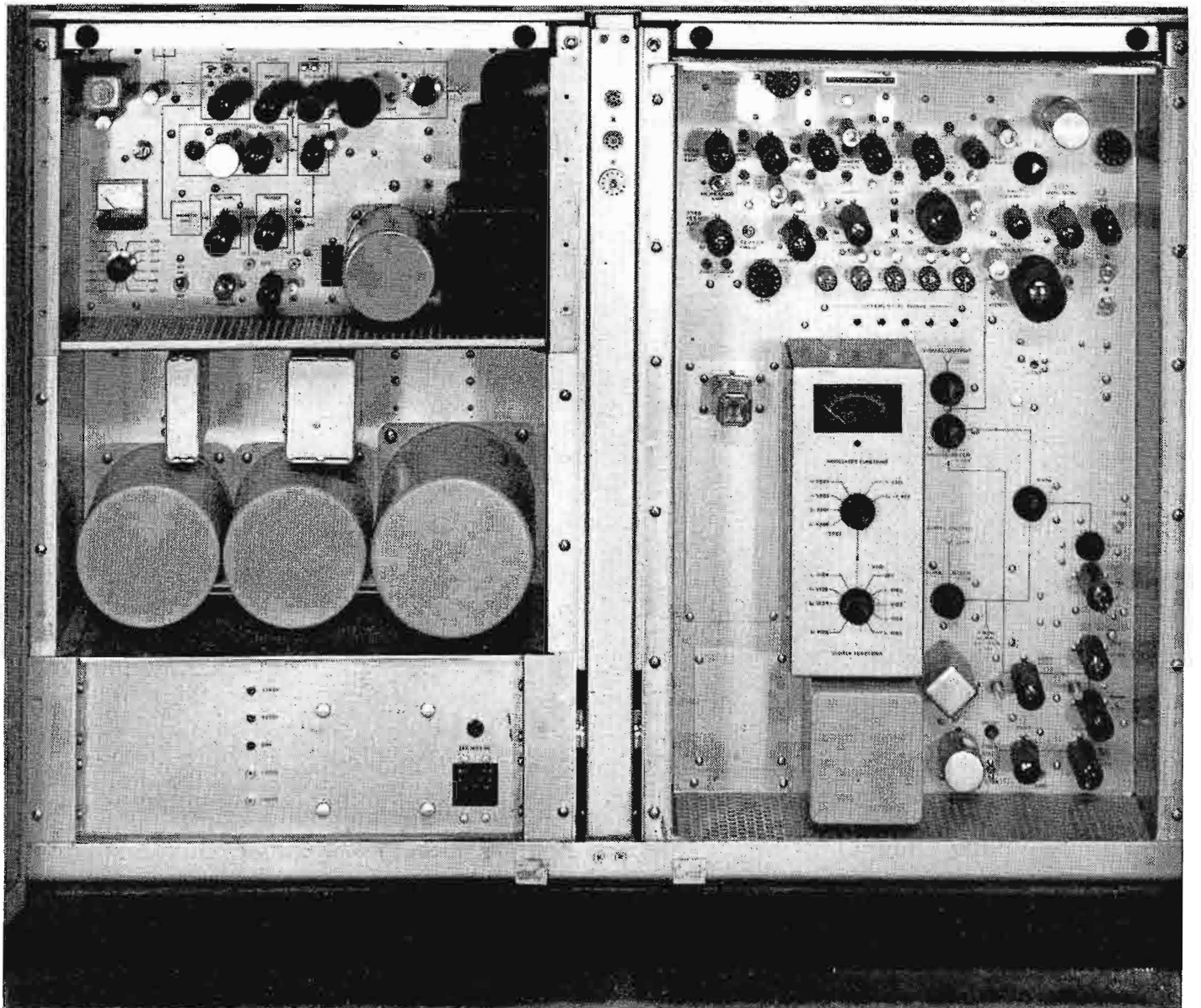
FIG. 6. Aural and visual exciter/modulator employs proven, high reliability circuits and 10,000 hour premium tubes.
