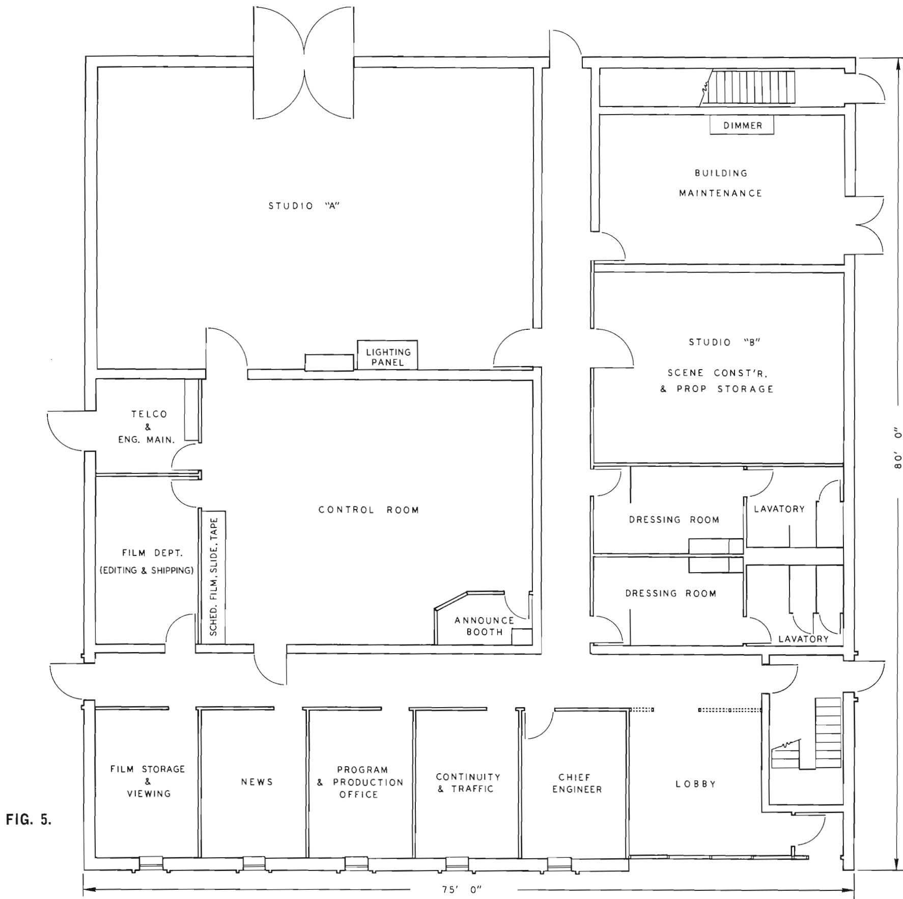
FIG. 5. Station first floor plan showing studios, control room, film handling areas, production facilities and offices.
