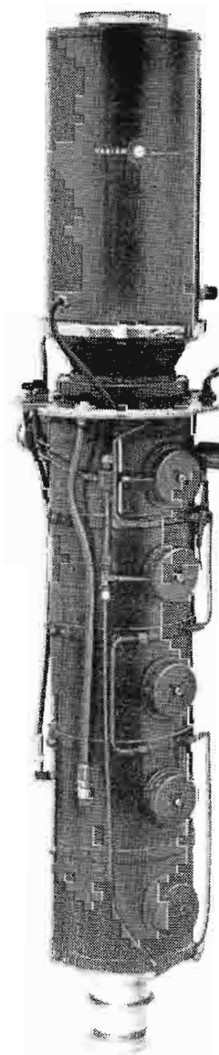
FIG. 4. Five-cavity, high power vapor cooled klystron features high efficiency and greater sensitivity than previous types.
