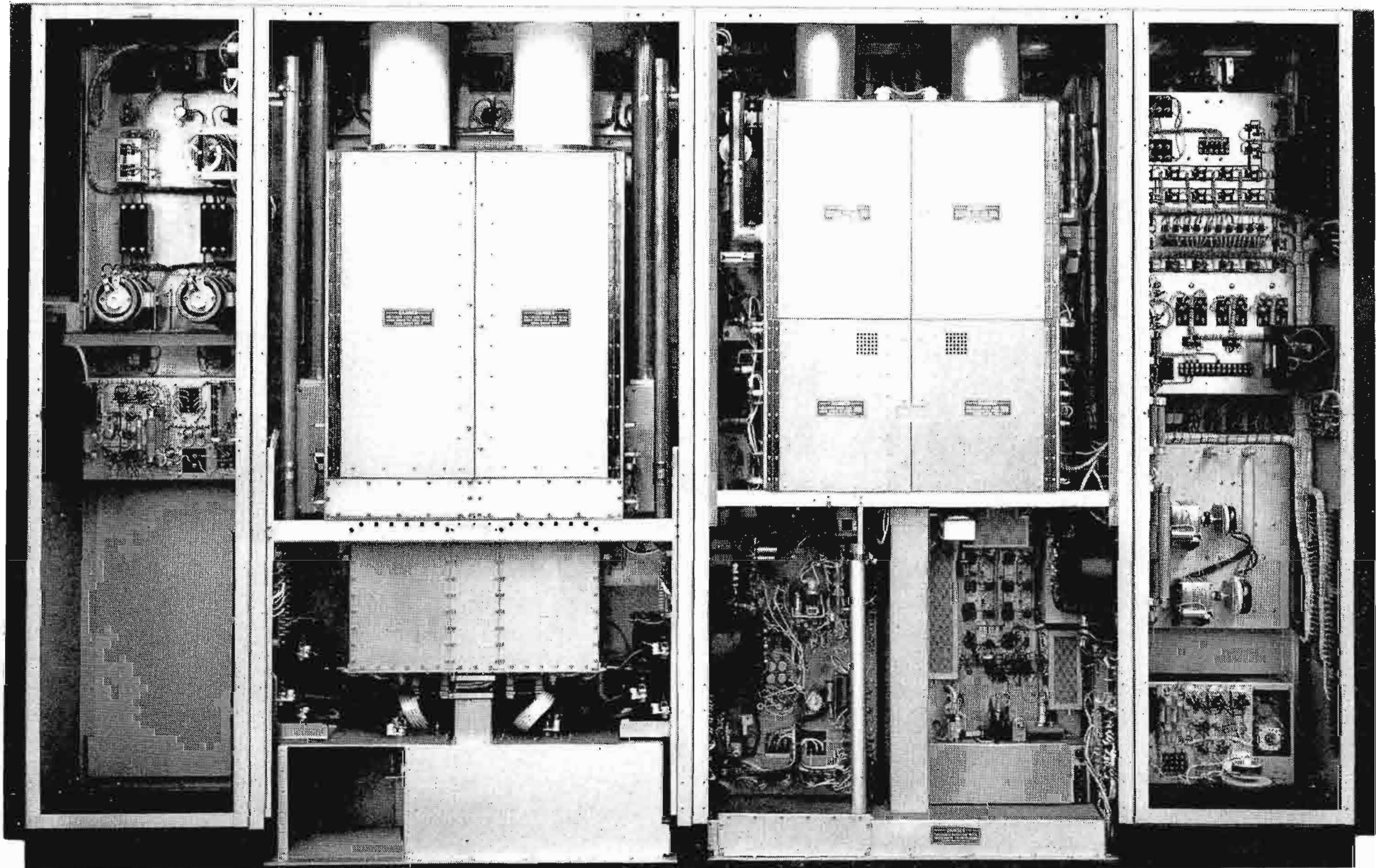
FIG. 6. Rear view of the TT-25EL VHF Transmitter showing from left to right the auxiliary control, diplexed 25 kW power amplifiers, 6 kW driver and transmitter control cabinets. Note the compact vertical construction which is completely accessible from the walk-in transmitter enclosure.
